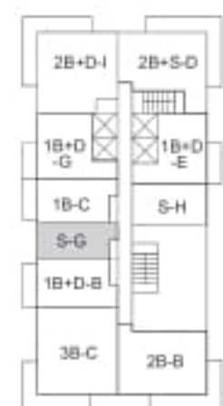
TOWER 2 LEVEL 10
