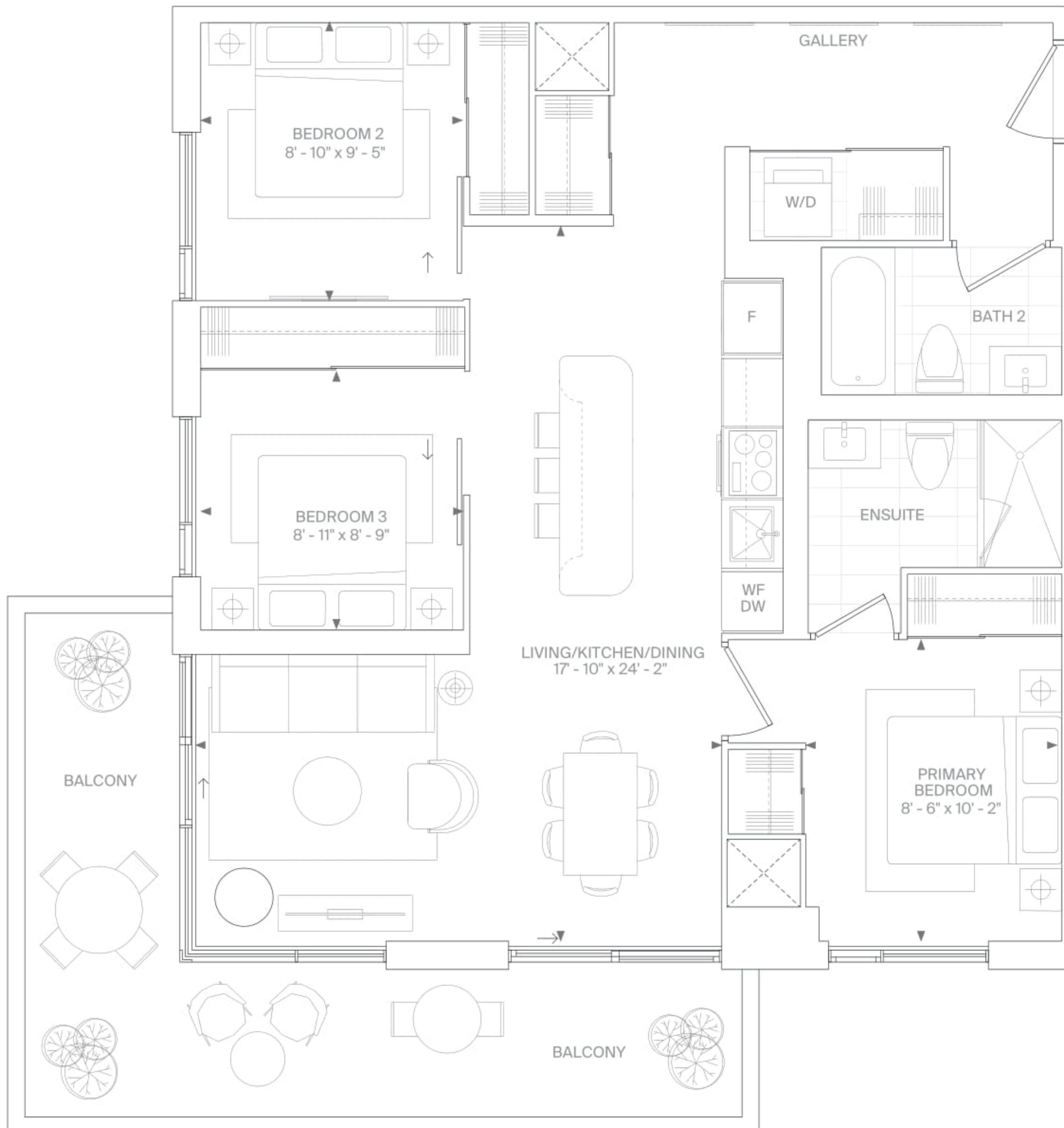
LEVEL 8, 10, 12, 14, 16, 18, 20, 22, 24, 26, 28 EXTERIOR 178 SF
