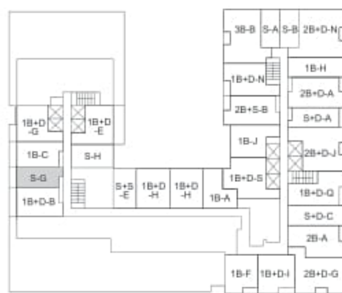
PODIUM LEVEL 6
