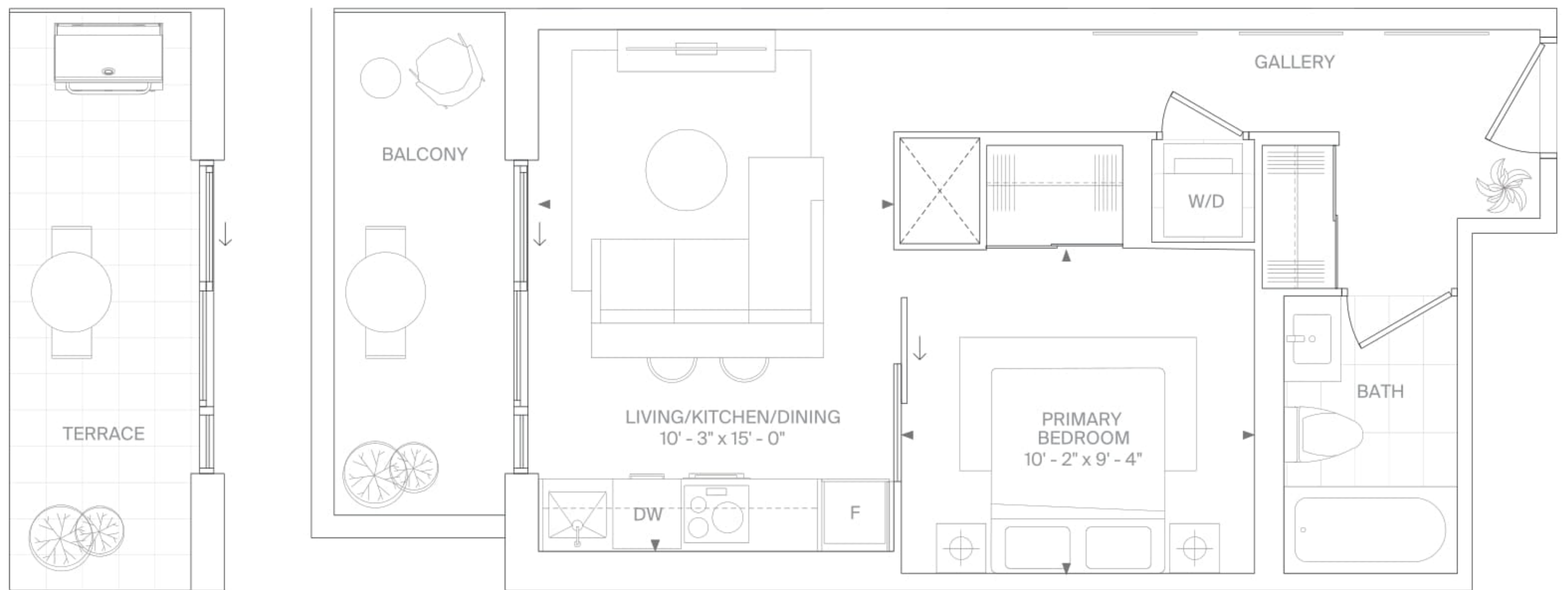
LEVEL 6 EXTERIOR 88 SF
