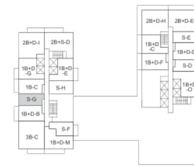
PODIUM LEVEL 9
