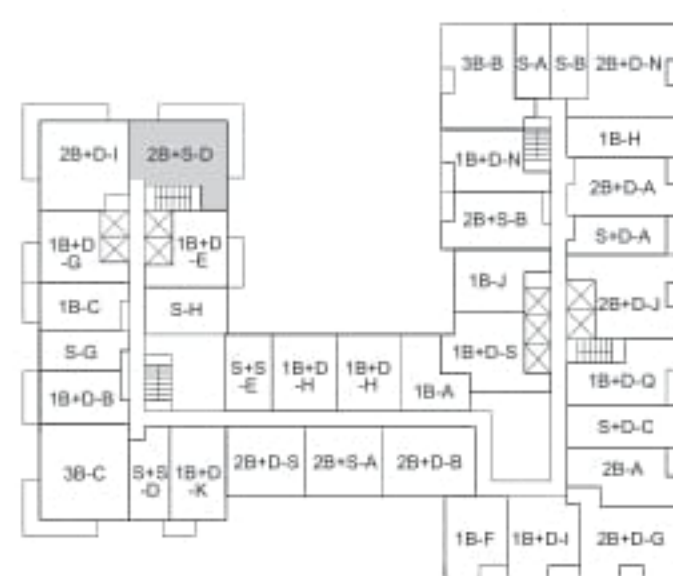
PODIUM LEVEL 8
