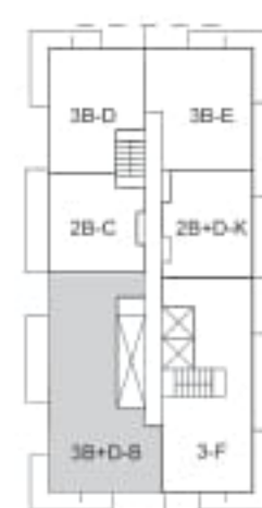
TOWER 3 LEVEL 23 - 24
